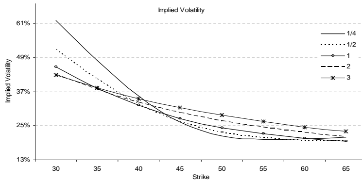
Figure 1: Implied volatility smile/skew curves as functions of the strike price for times to maturity from 1/4 to 3 years. Current stock price level is 50.
