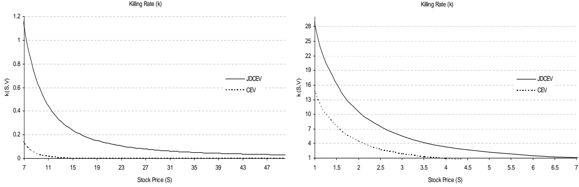
Figure 3: Killing rate (default intensity) k(S, V) as a function of the stock price S when the activity rate is fixed at V = 1 . The solid line is the default intensity in the model obtained by time changing the JDCEV process. The dashed line is the default intensity obtained by time changing the standard CEV process with b = c = 0 without the jump to default (see Remark 8.4).
